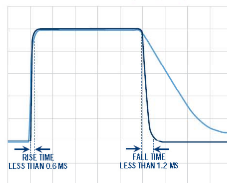
TYPICAL PULSE IN CINE @ 30 f/s, 100 kV, 32 mA, 12.5 ms
